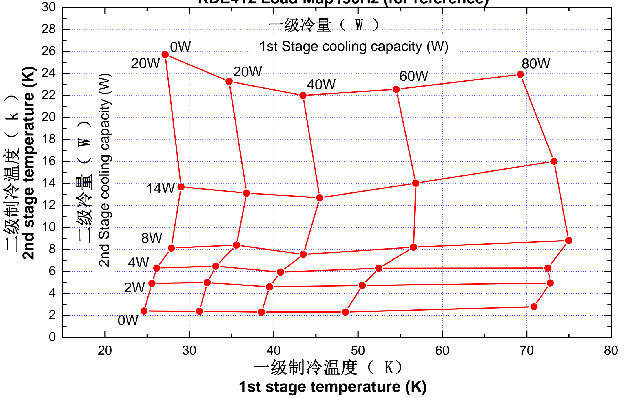
KDE412制冷机制冷量/50Hz (参考) KDE412 Load Map /50Hz (for reference)
